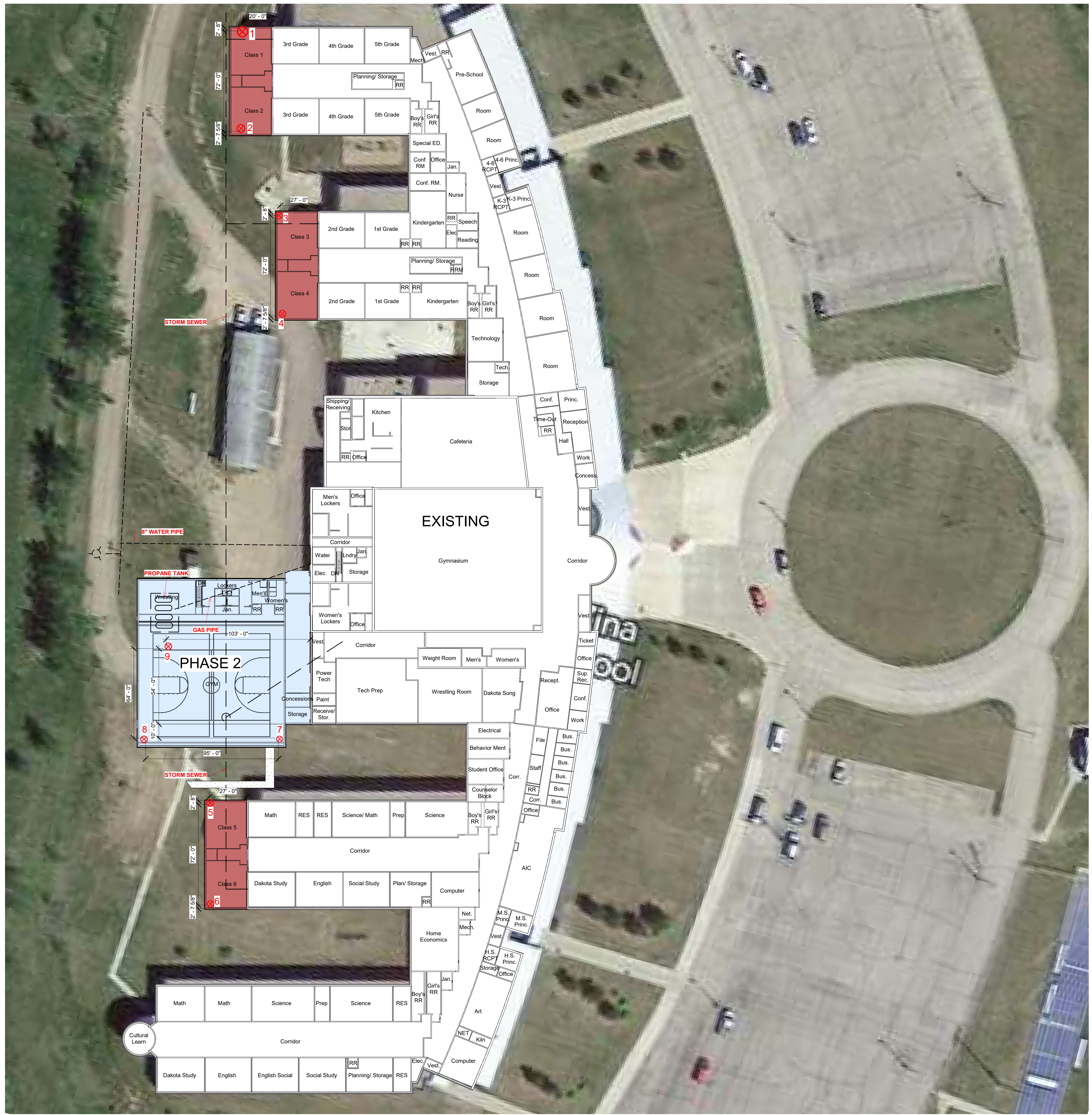
1 Site 1" = 30'-0"
